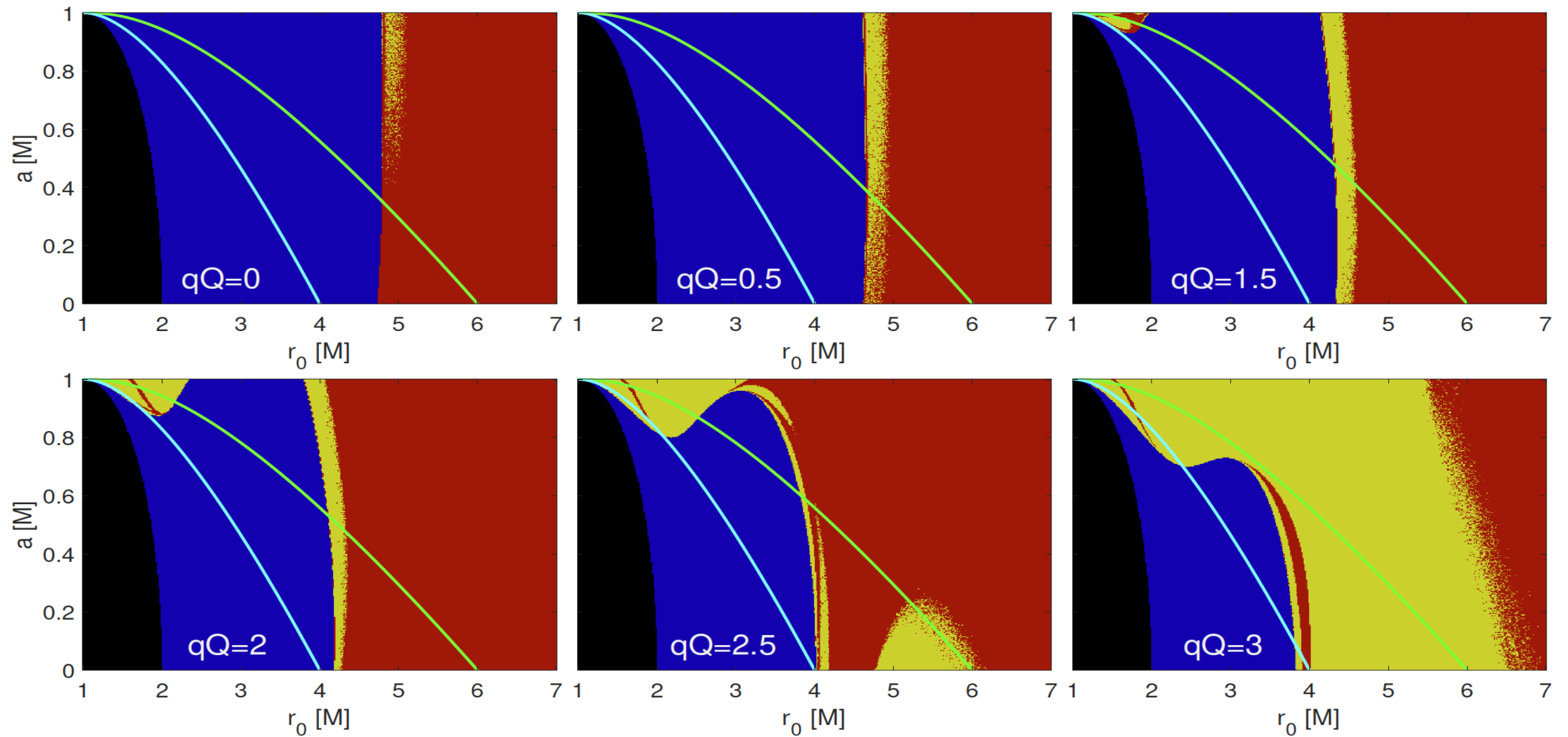
Figure 1. Evolution of escape zones of charged particles affected by the Coulomb repulsion of charged black hole. Color-coding of trajectories: blue for plunging orbits, red for stable ones (bound to the black hole) and yellow for escaping trajectories. The inner black region marks the horizon of the black hole. The green line denotes the ISCO of neutral particles, while the cyan line marks MBSO. Parameters of the system are qB = -1 and inclination \alpha = 0 while qQ varies as indicated.
