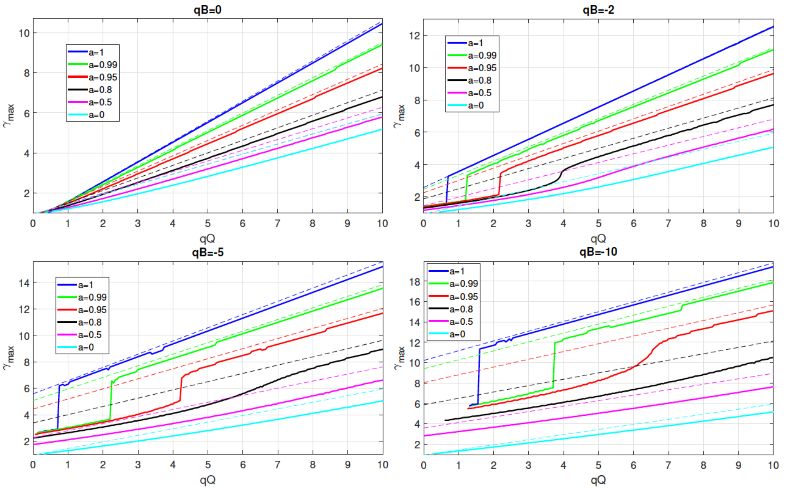
Figure 3. Maximum Lorentz factor achieved within the escape zones as a function of charge product qQ compared with a theoretical limit for given values of parameters, as determined by eq. (21) (dashed lines).
