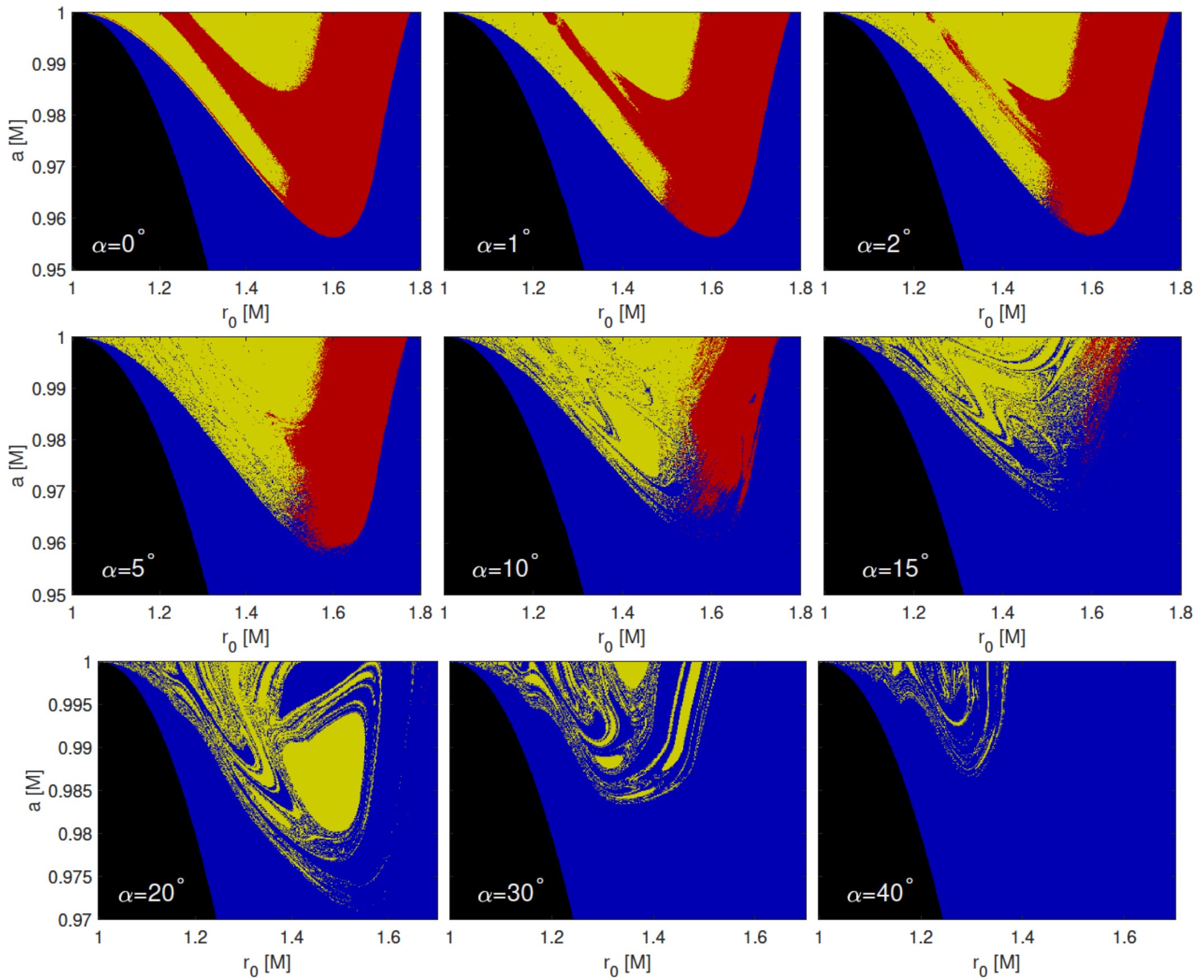
Figure 5. The Innermost Escape Zone affected by the inclination of the magnetic field. Color-coding of trajectories is the same as in Fig. 1. Parameters of the system are qB = -1 , qQ = 1.2 , \varphi(0) = 0 , and inclination angle \alpha varies as indicated.
