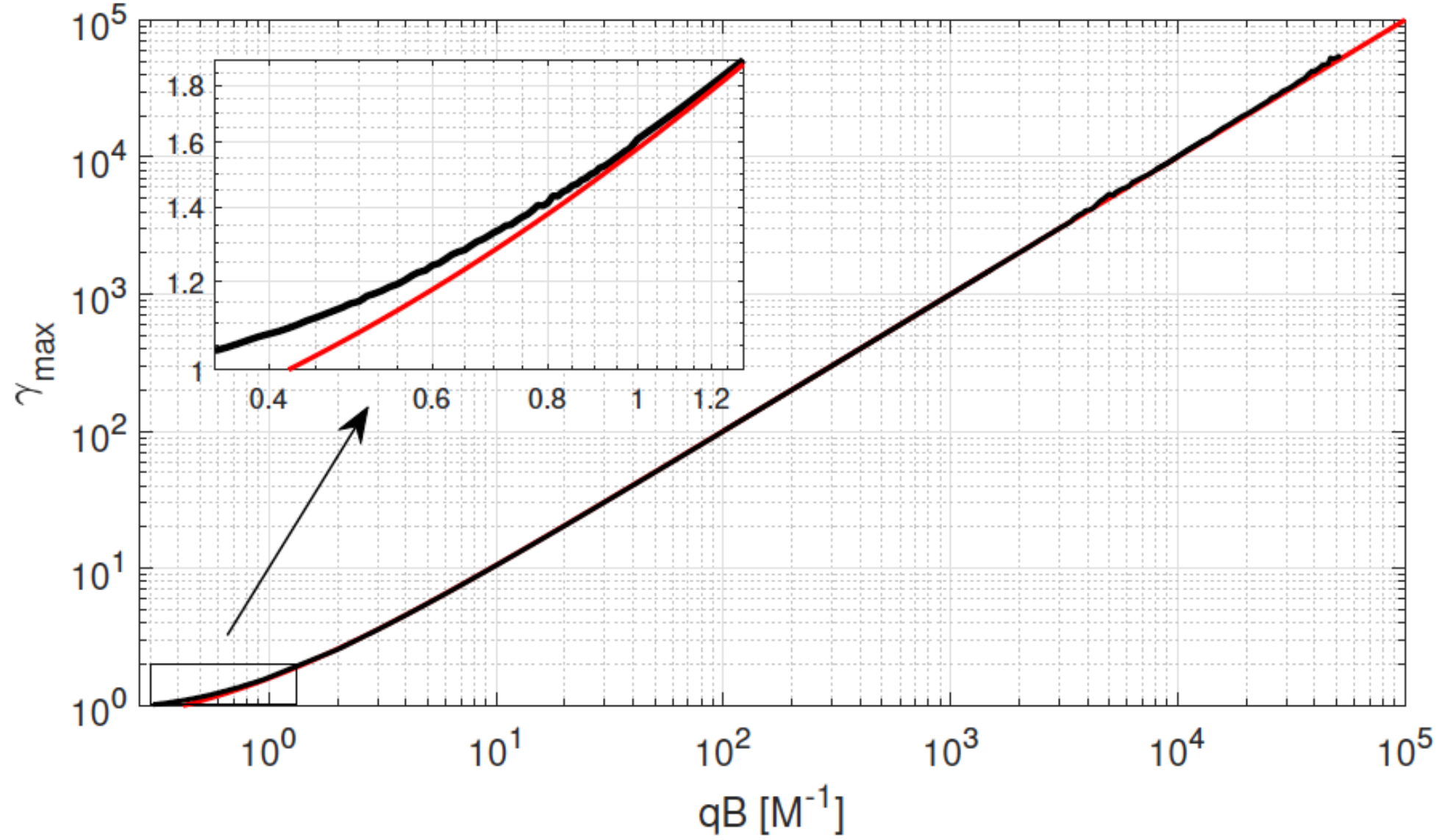
Figure 10. Maximal value of the final Lorentz factor of escaping particles from the vicinity of the Kerr black hole with Wald charge as a function of parameter qB . Numerically obtained actual values detected within escape zones (black) vs. estimated theoretical maximum (red).
