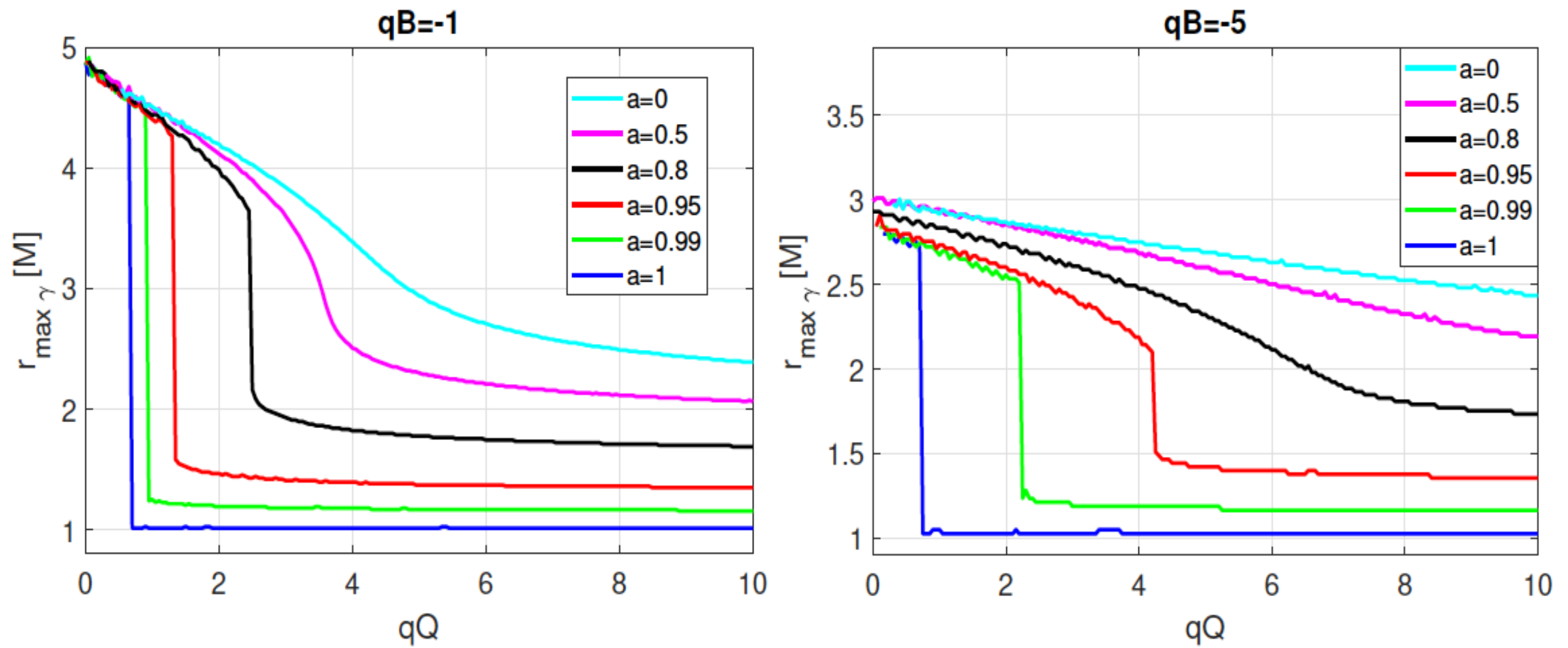
Figure 4. Values of initial radial coordinate of maximally accelerated escaping particle within escape zone as a function of charge product qQ .
